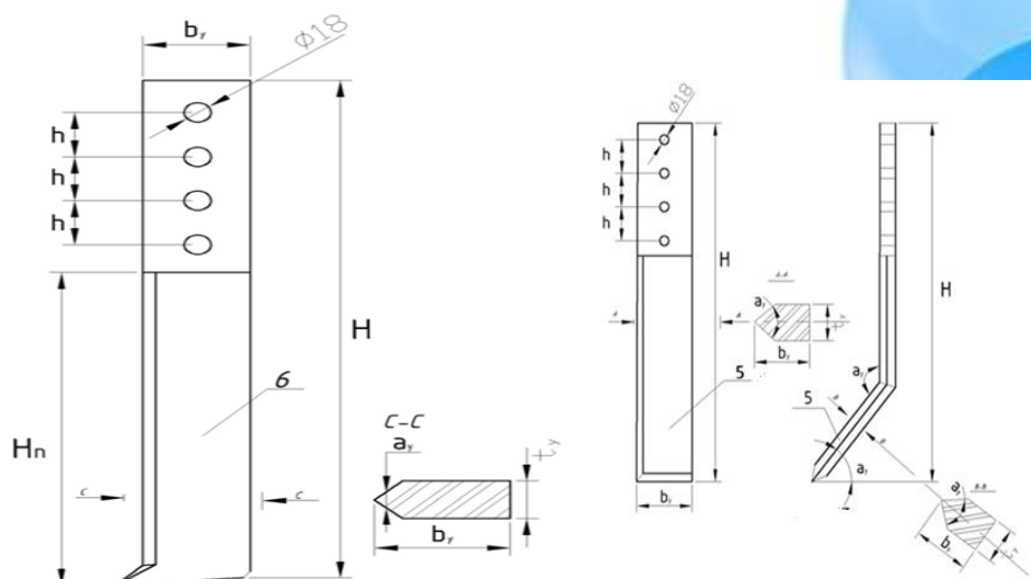
Figure 2. Advanced perforated drainage forming device middle and side work columns
